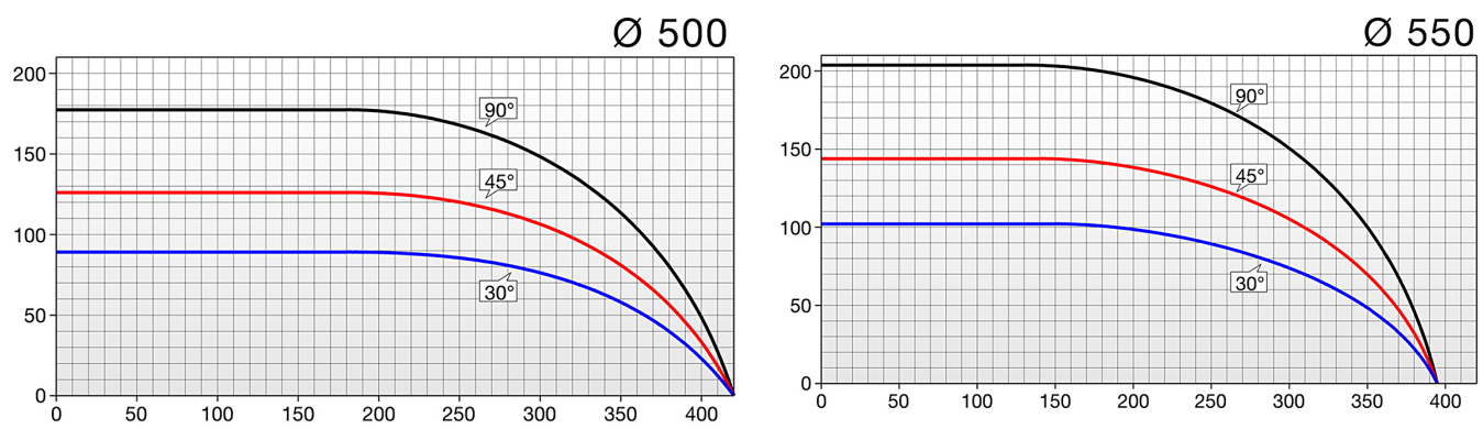
Cutting chart
